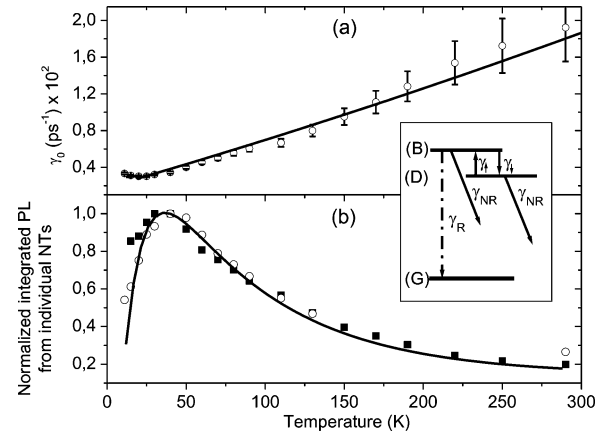
Figure 3. (a) Internal decay rate \gamma_0 (open circles) of the (9,4) SWCNT as a function of temperature. The solid line is the computed internal decay time from the three level model. (b) Normalized integrated photoluminescence signal (black squares) from isolated nanotubes (corresponding to the j = 0 component in eq 1) and corresponding fraction in PL measurements under CW excitation (open circles). The solid line is the computed PL intensity from an individual nanotube in the three level model. (Inset) Schematic of the three-level model.
