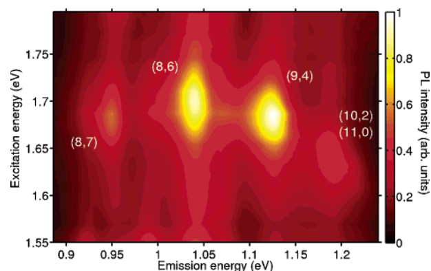
Figure 1. Photoluminescence intensity at 10 K of isolated HiPCO SWCNTs embedded in a gelatin matrix plotted as a function of emission and excitation energies. By comparison to the semiempirical Kataura plot, PL spots are assigned to a given SWCNT chirality.
