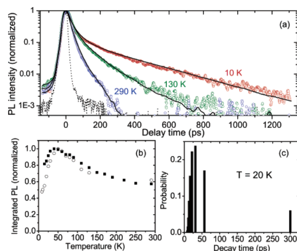
Figure 2. (a) Time-resolved photoluminescence of isolated (9,4) SWCNTs in a gel on a semilogarithmic scale for an excitation at 1.7 eV. System response function (dotted line) obtained from the elastic scattering of the laser: The temporal resolution is 26 ps. Normalized photoluminescence transients (open circles) are well reproduced by the convolution (solid lines) of the model I(t) (eq 2) and the response function. (b) Normalized integrated PL signal as a function of the temperature (black dots); normalized CW PL signal (open circle). (c) Probability distribution of lifetimes at 20 K.
